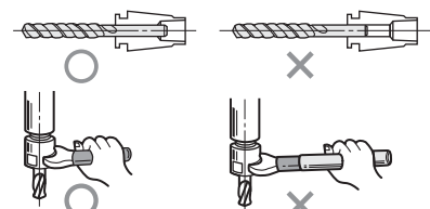
Slim Chuck
