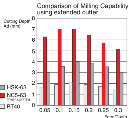
Comparison between HSK-63, NC5-63 & BT40
